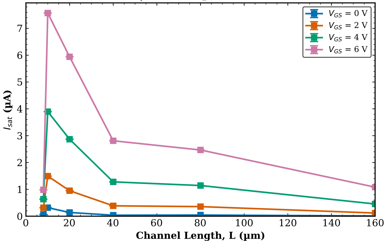
TFT1 Transistor 1 I_{sat} vs L | W = 10 \mu\text{m} (mean \pm std)
